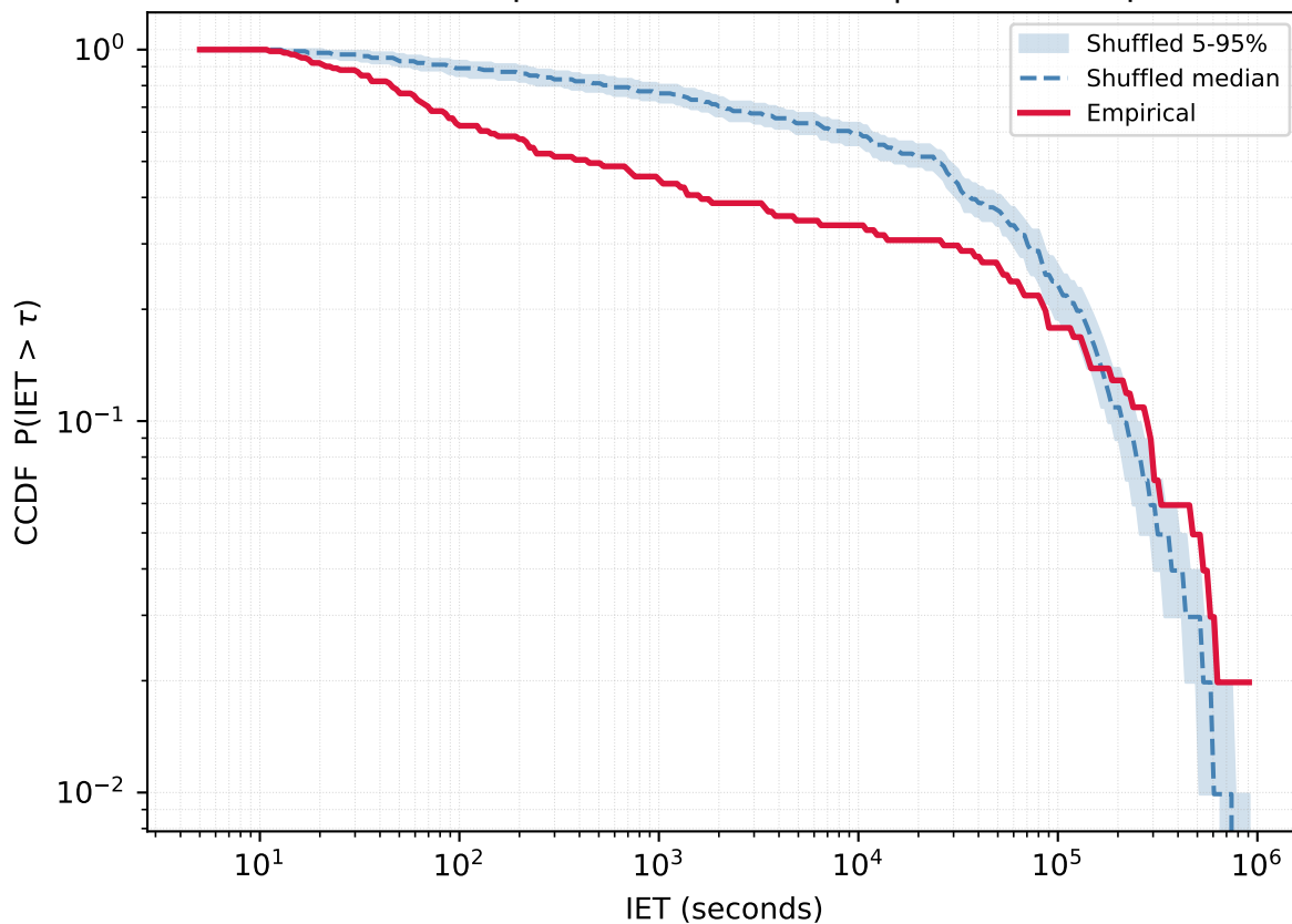
User 5357949 - Empirical vs Reshuffled | KS=0.346 p=0.000
